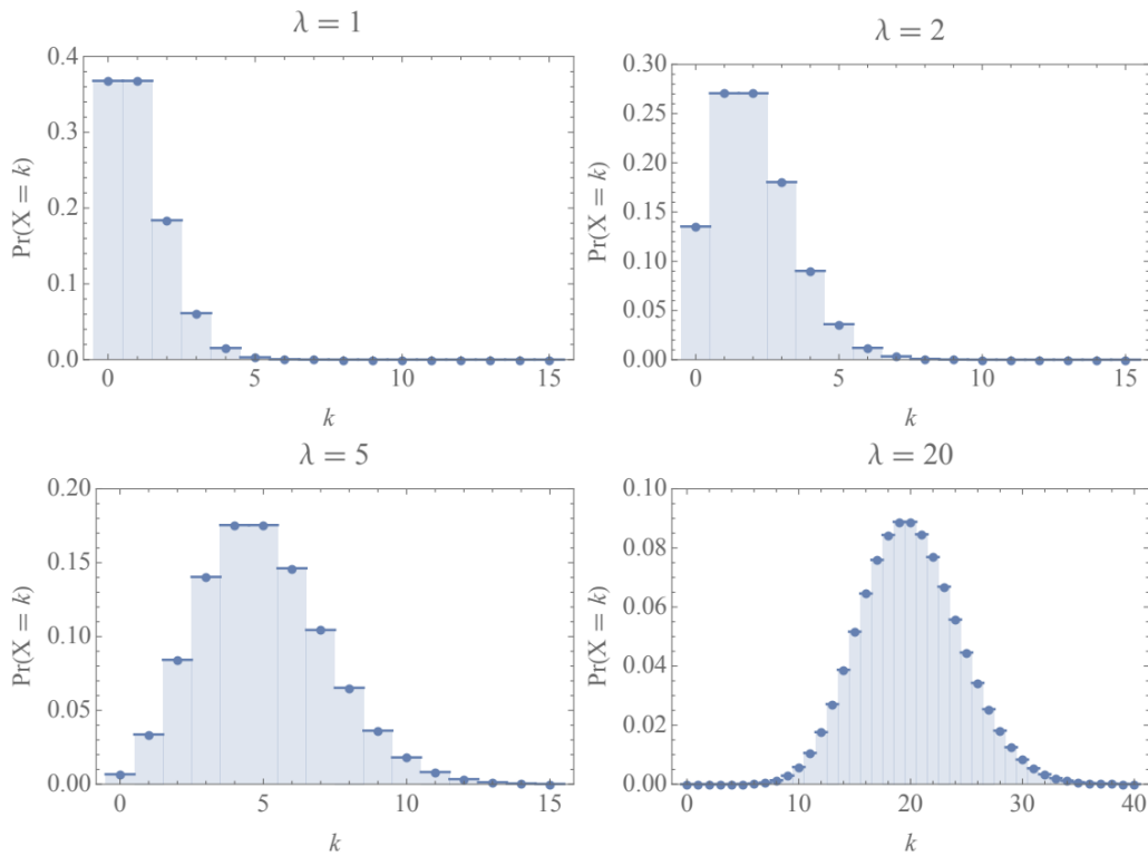
Figure 2: Illustration of the \text{Poisson}(\lambda) distribution for \lambda = 1, 2, 5, 20 .
